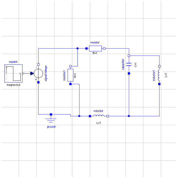
Figure C.4. Electric Circuit
